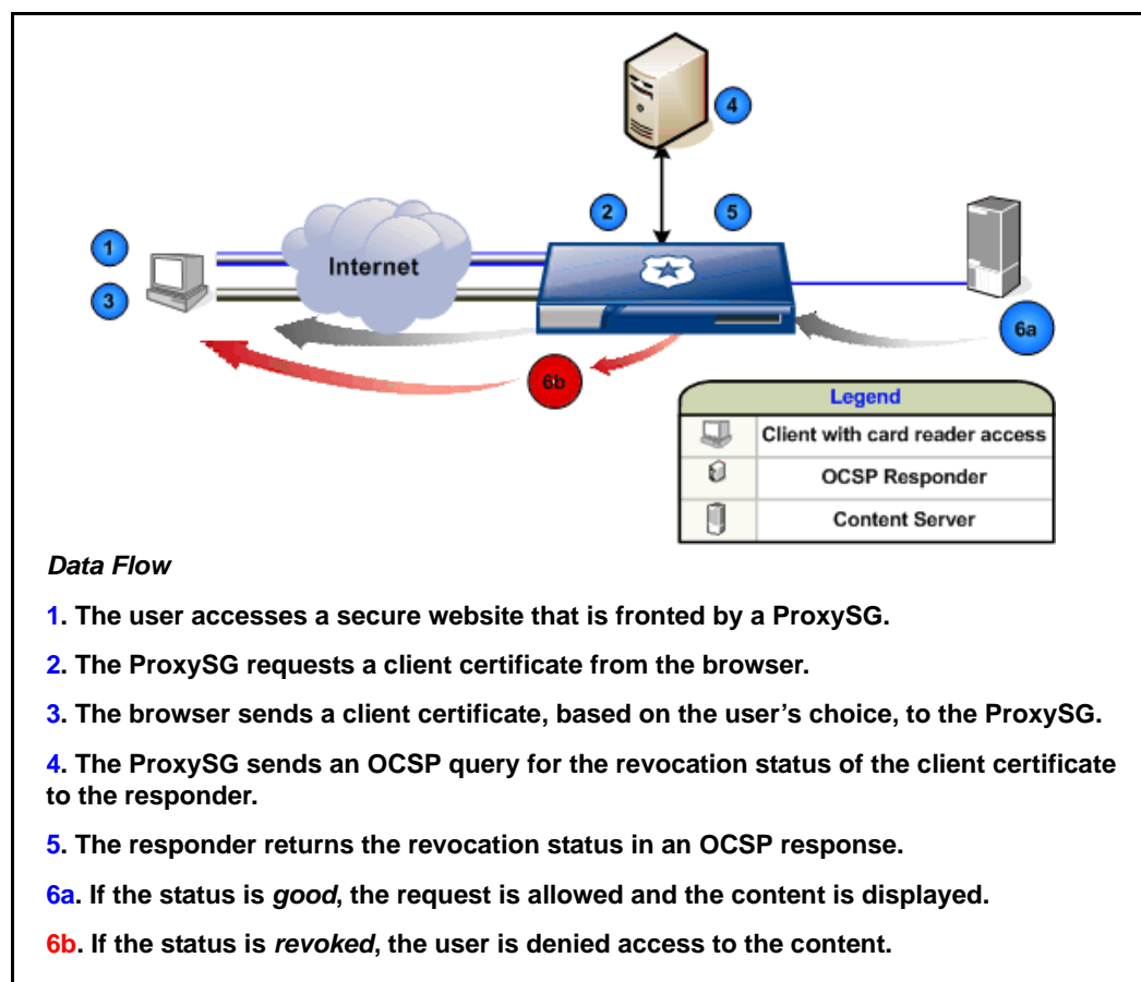
Figure 4-1 Reverse Proxy Scenario
